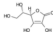
5. L-ascorbic acid (Vitamin C)
