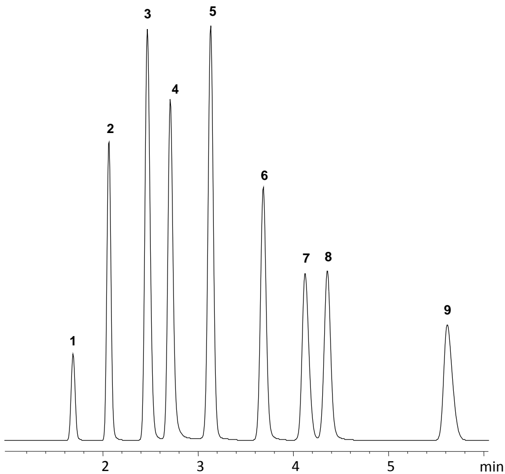
5. L-ascorbic acid (Vitamin C)
