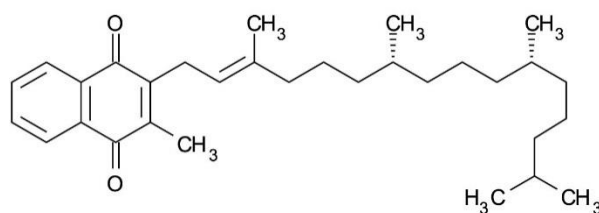
2. trans -Vitamin K1 (2,3- trans -phyloquinone)
