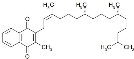
2. cis -Vitamin K1 (2,3- cis -phyloquinone)
