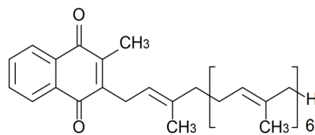
3. Vitamin K2 (MK-7) – Menaquinone 7
