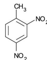
4. 2,4-Dinitrotoluene
