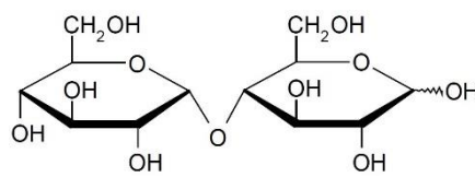
2. Maltose
