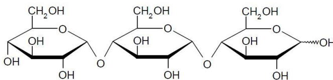
3. Maltotriose
