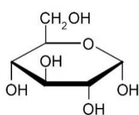
1. Glucose
