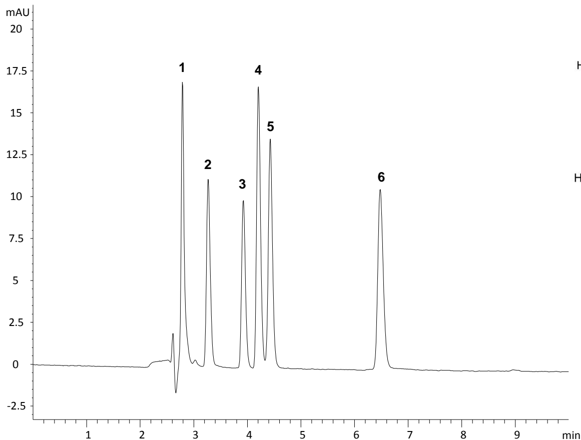
2. Tartaric acid
