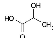
4. Lactic acid
