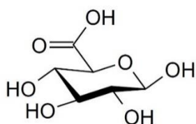
1. Glucuronic acid
